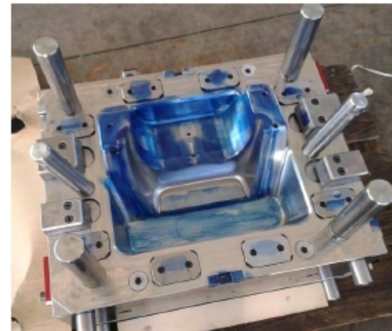
Mould matrix "Mostrina mobiletto Fint 520" steel
